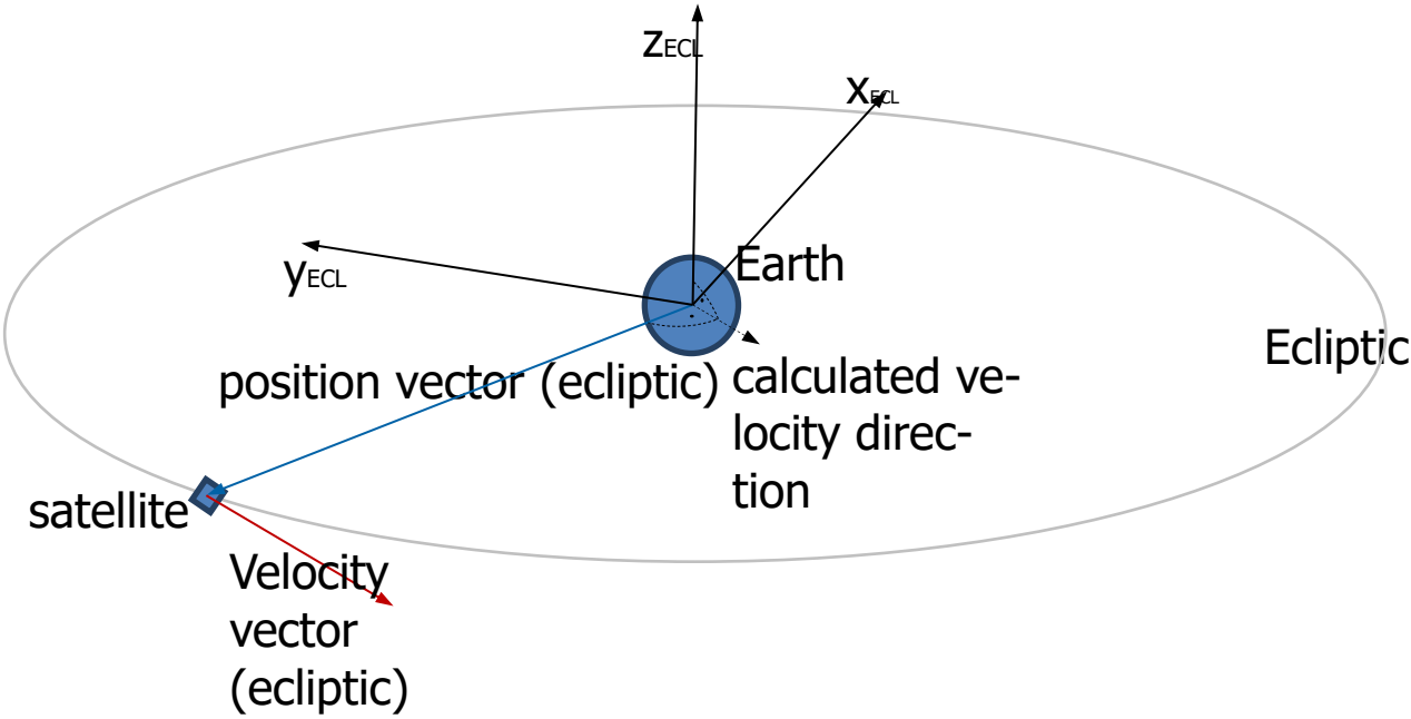
Figure 6-4 Schematic illustration of the calculated state vector in ecliptic coordinate system.
