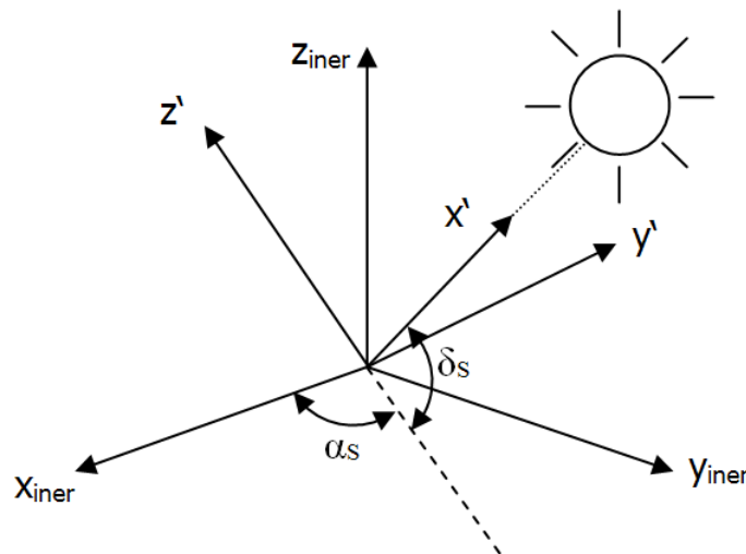
Figure 7-1 Selenocentric inertial ( _{iner} ) to EARTHLEQ ( ' ).
